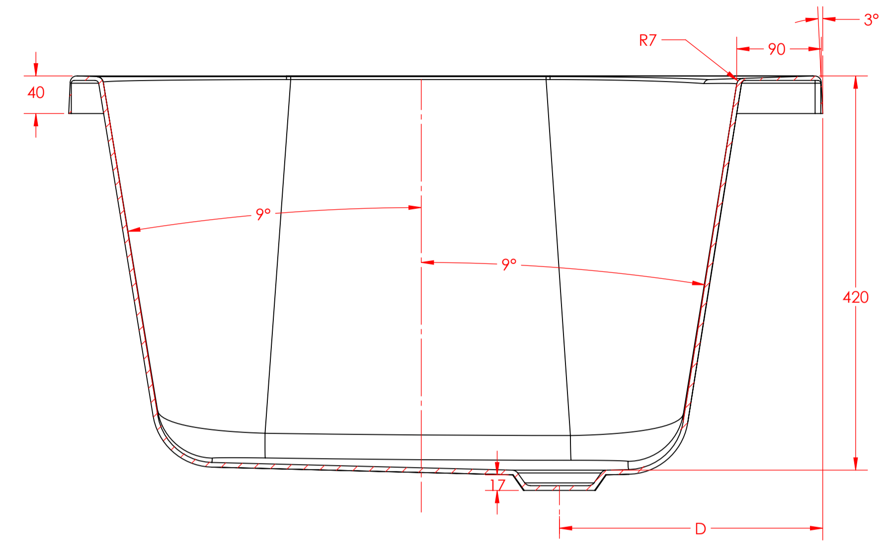
SECTION C-C SCALE 1 : 4
